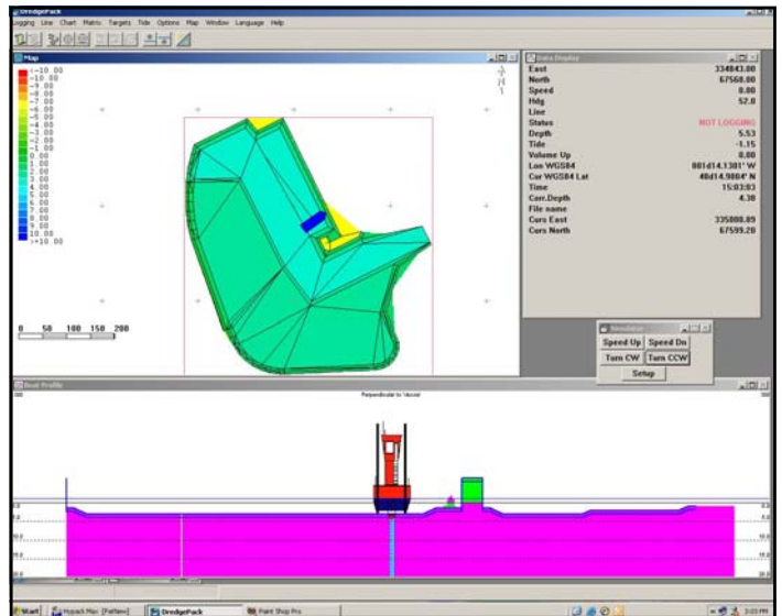
A real time cross section through the complex dredging plan.
