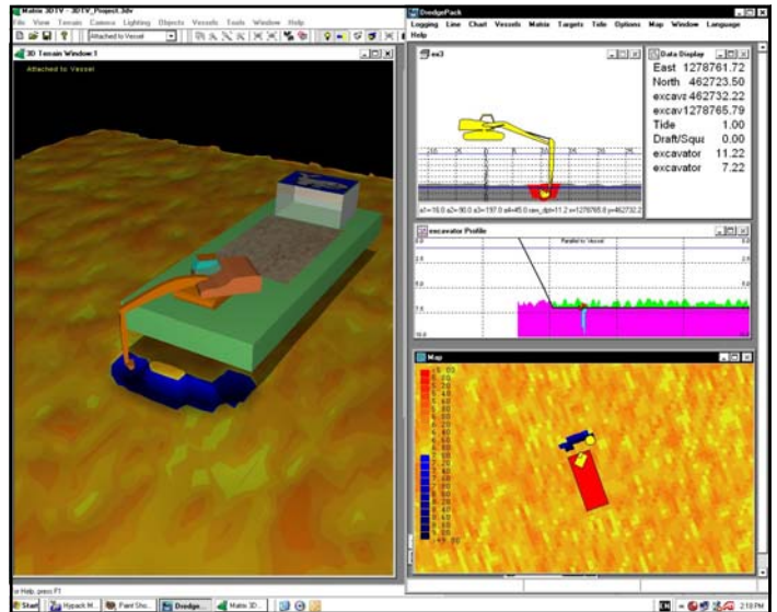
3D Visualization with an excavator integrated in DREDGEPAK ® .
