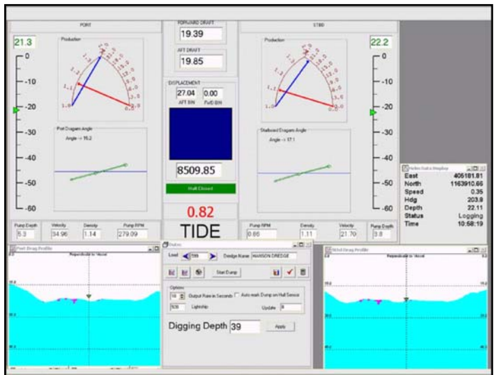
Customized display for hopper dredge using OPC Network.
