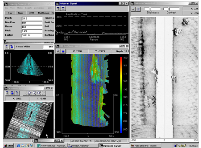
Real time collection display from HYSWEEP® SURVEY.
