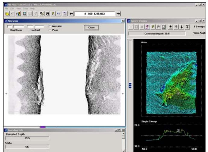
Editing swath data with backscatter imagery displayed in the MULTIBEAM EDITOR of HYSWEEP®.
