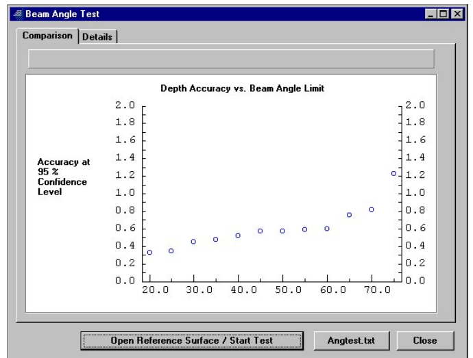
The Performance Test results from HYSWEEP® show the repeatability of your system versus beam angle.
